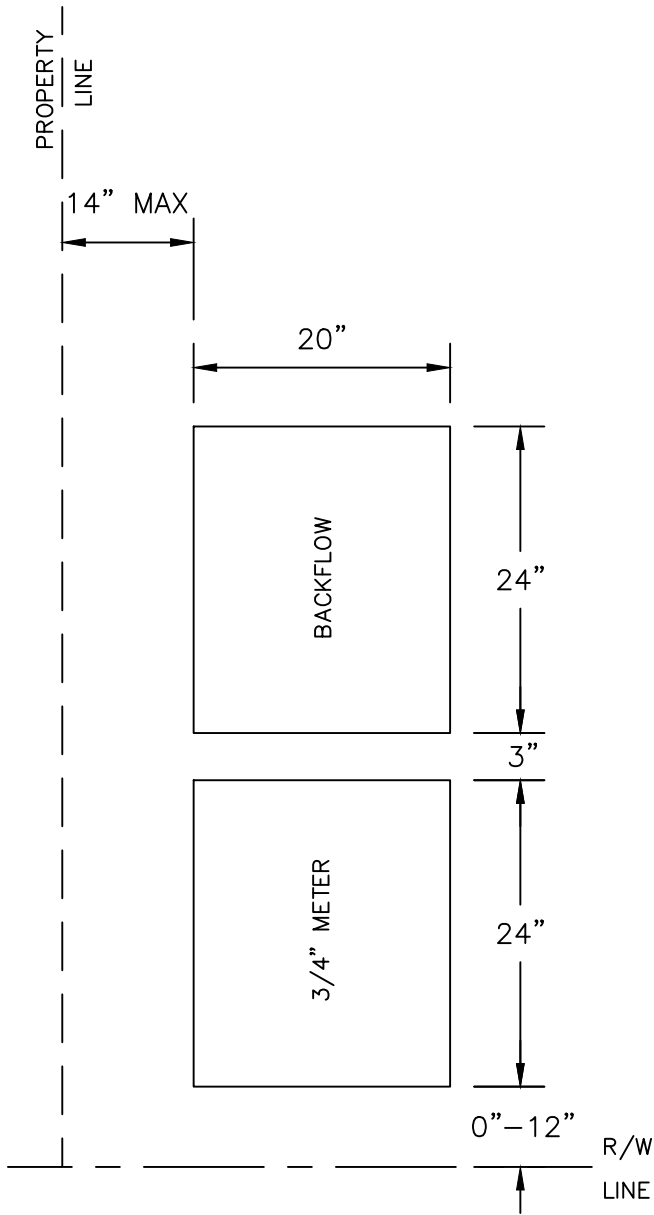
SINGLE BOX WATER METER WITH BACK FLOW PREVENTER
