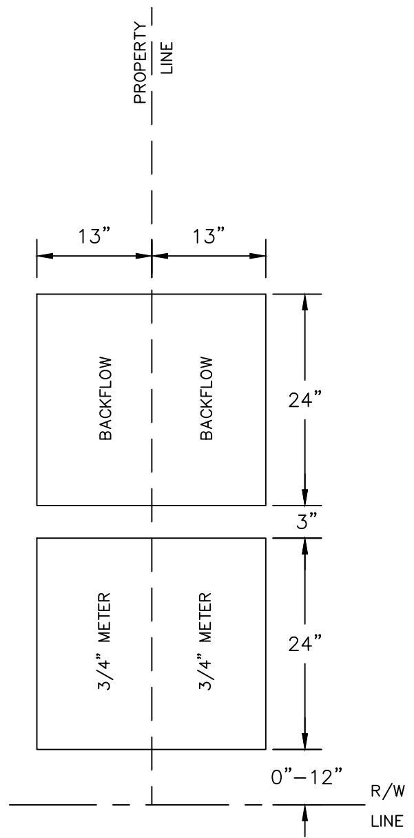
DOUBLE BOX WATER METERS WITH BACK FLOW PREVENTERS
