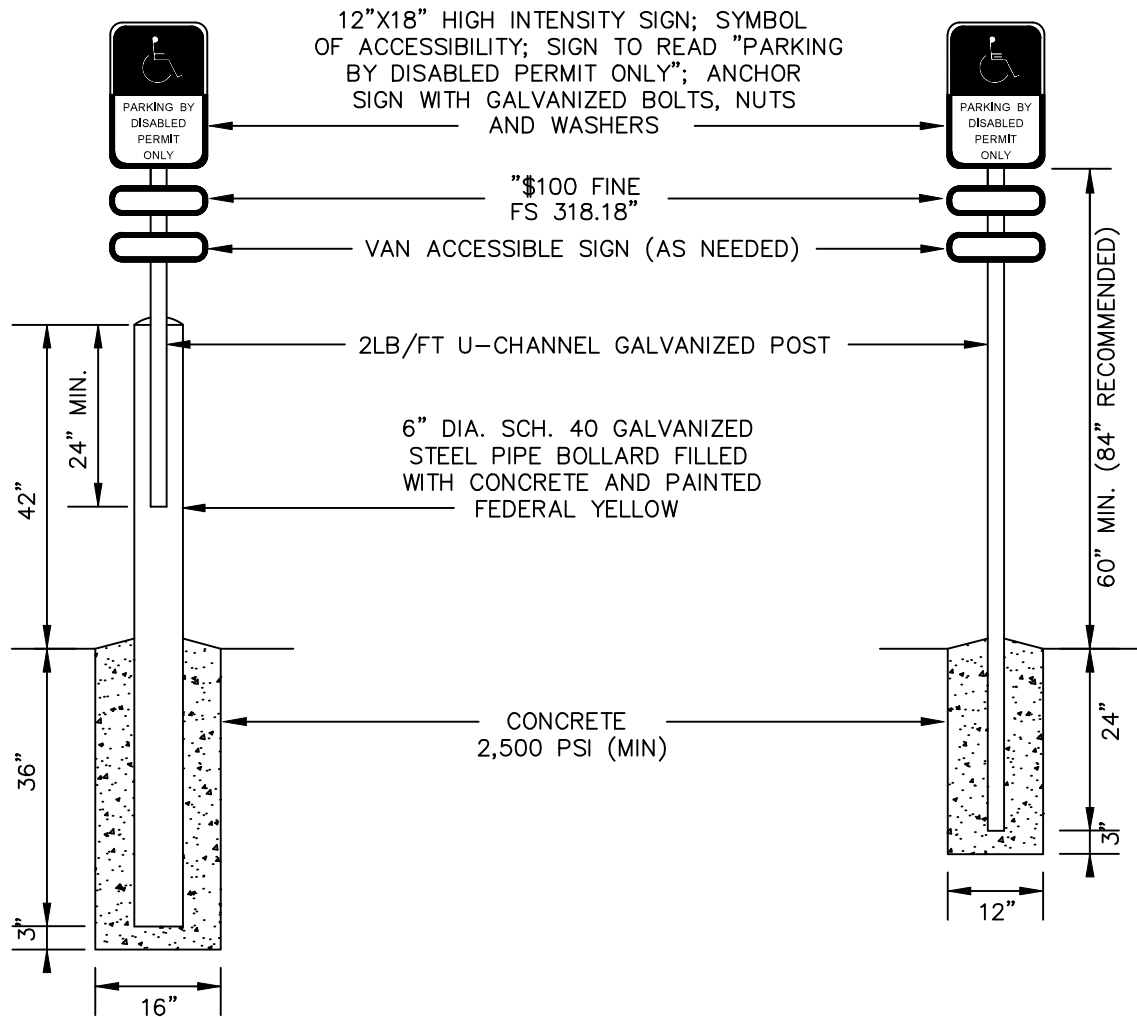
BOLLARD/SIGN COMBINATION
